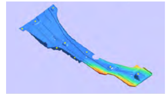
LEFT: CAD model of air deflector TOP: Modal reference result obtained with current solver BOTTOM: Modal result obtained with Altair SimSolid
